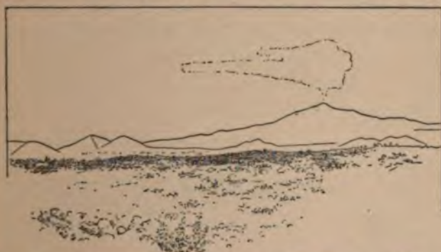
125.—View looking toward the summit of Etna from a position upon the thern flank near the village of Nicolosi. The two breached parasitic cones n behind this village are the Monti Rossi which were thrown up in 1669 and m which flowed the lava which overran Catania (after a photograph by umer).
